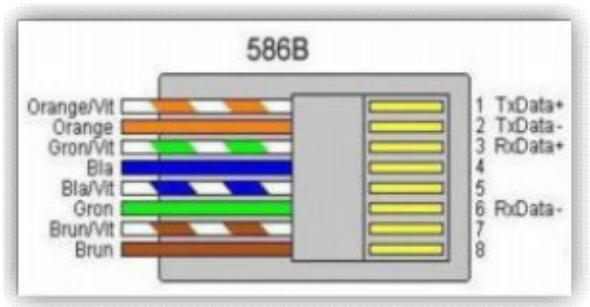
Figure 3 Ethernet cable
